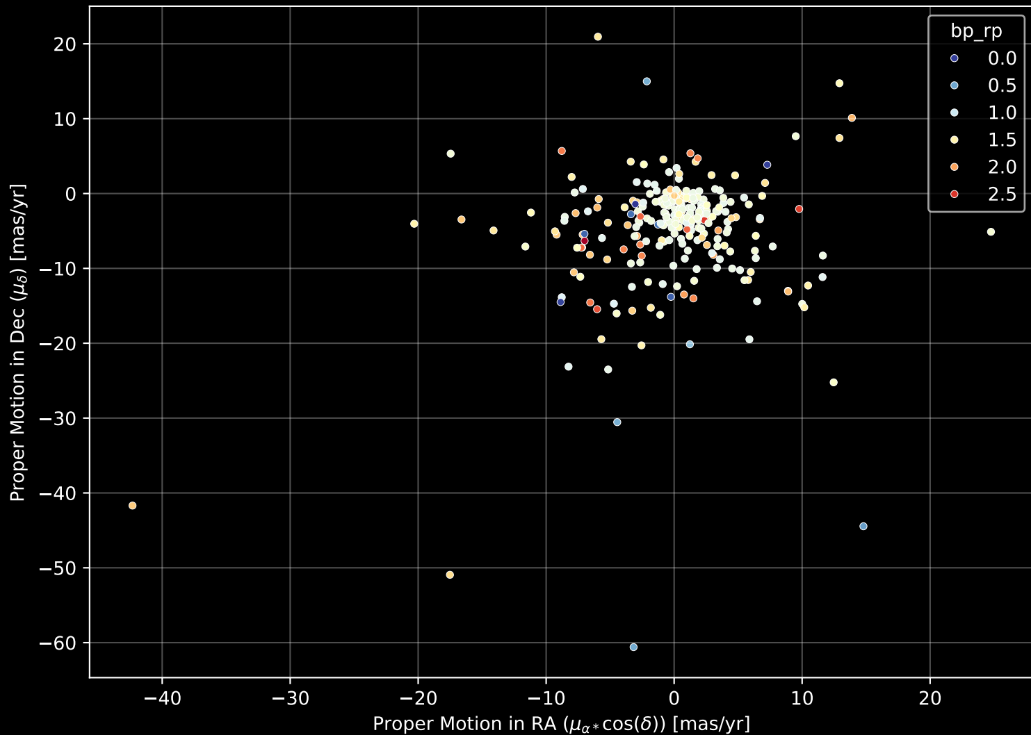
APOGEE DR17 Field: [160+24_btx] Proper Motion Diagram (n= 288)
