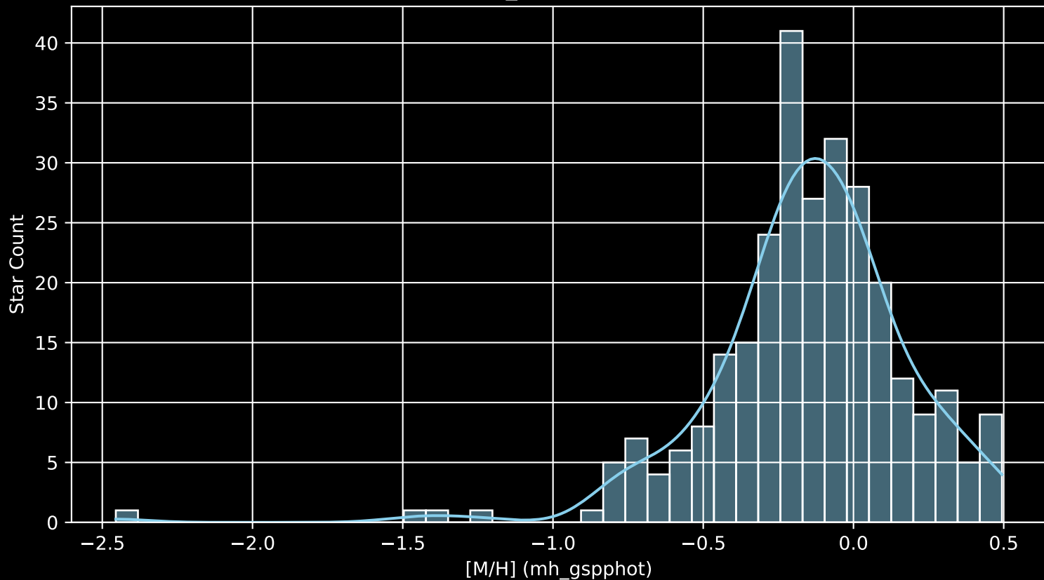
APOGEE DR17 Field: [160+24_btx [M/H] (mh_gspphot) (n= 282)
