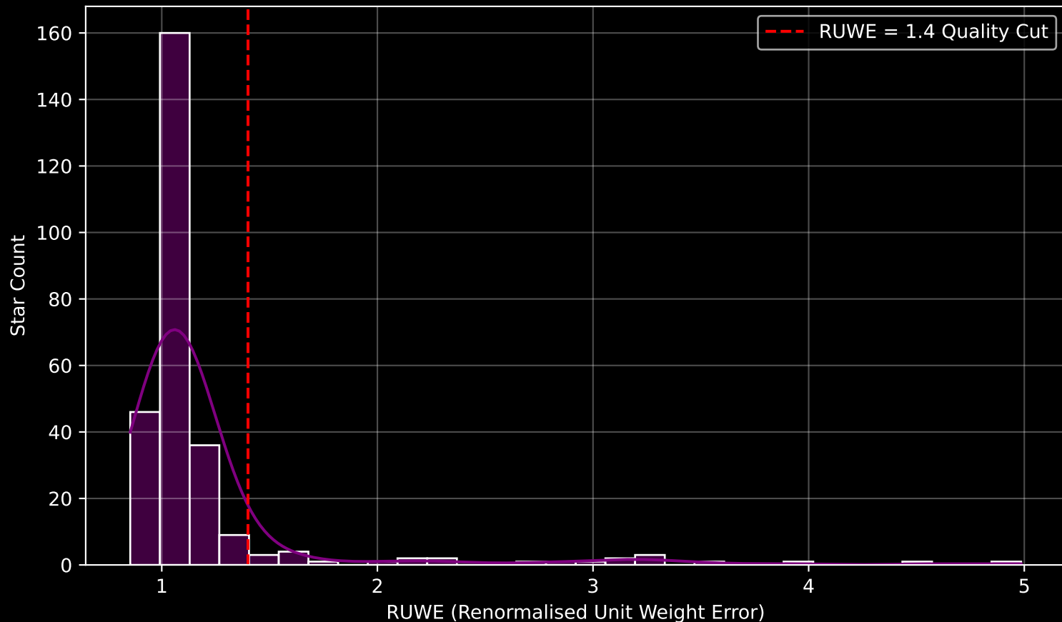
GAPOGEE DR17 Field [160+24_btx] RUWE Distribution (n= 276)
