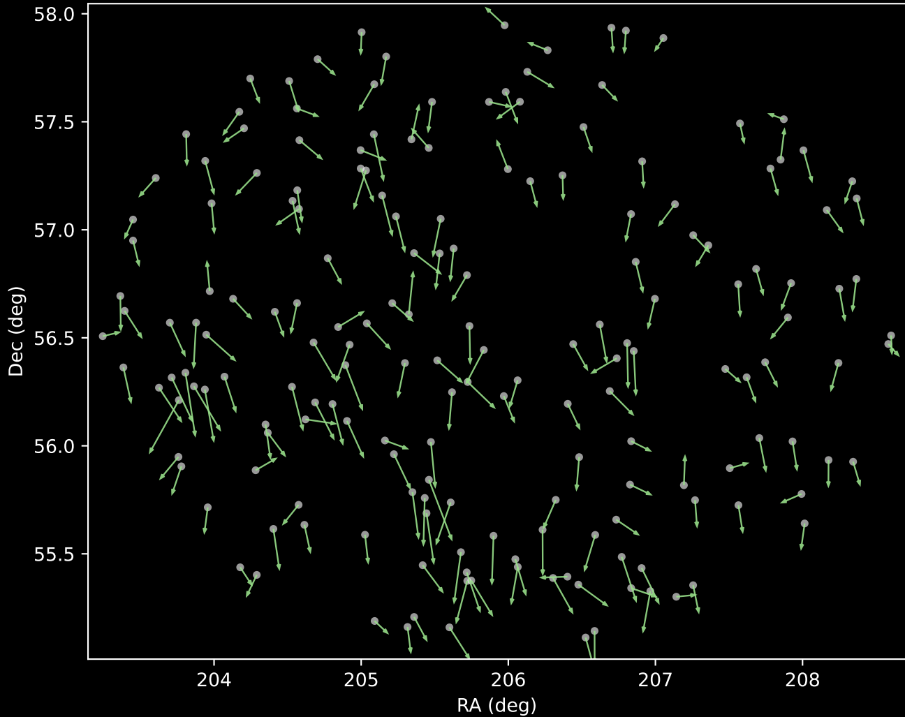
APOGEE DR17 Cluster 5 Proper Motion Vectors (n=181)
