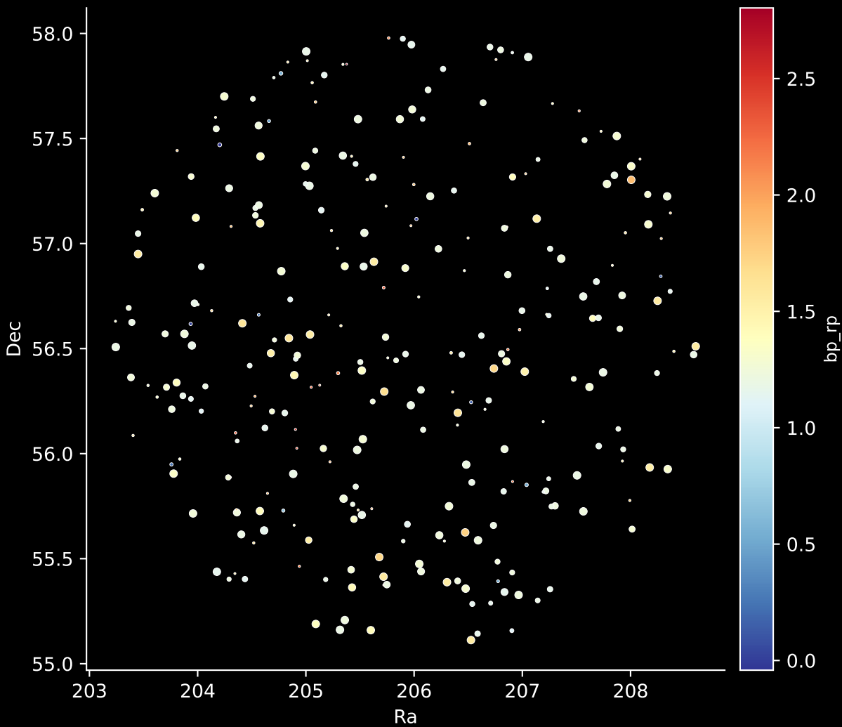
APOGEE DR17 Field: [160+24_btx] Stars: 288
