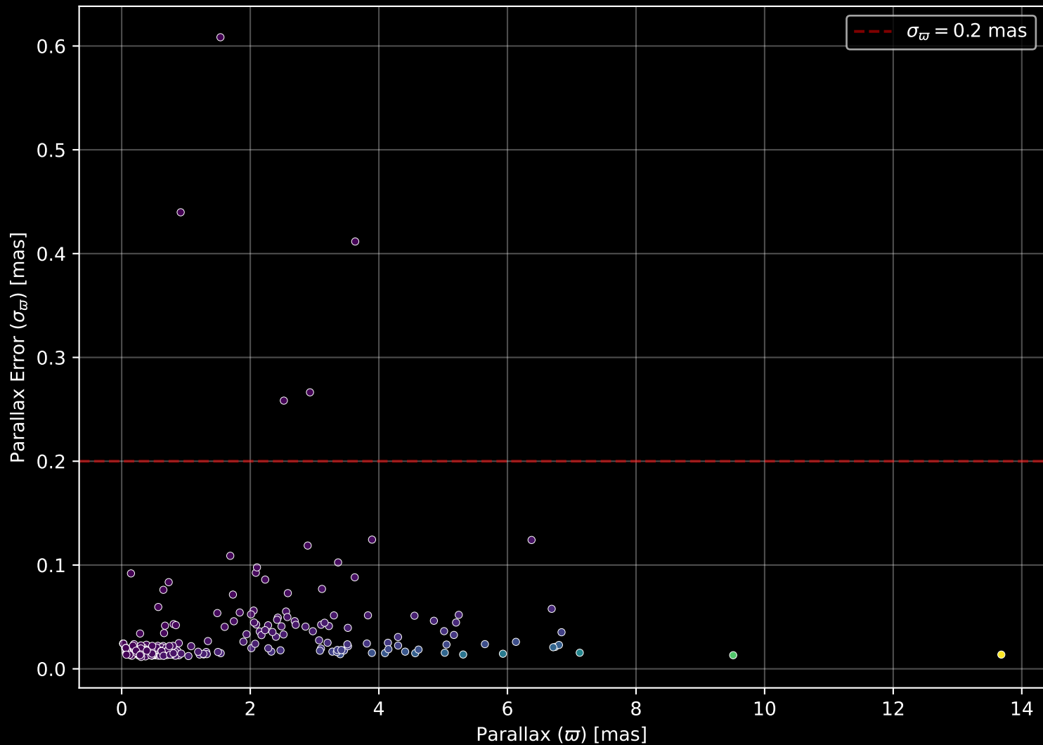
APOGEE DR17 Field: [160+24_btx] Parallax Quality (n= 288)
